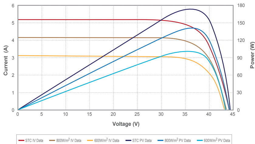
CurrentPower v.s. Voltage Characteristics
